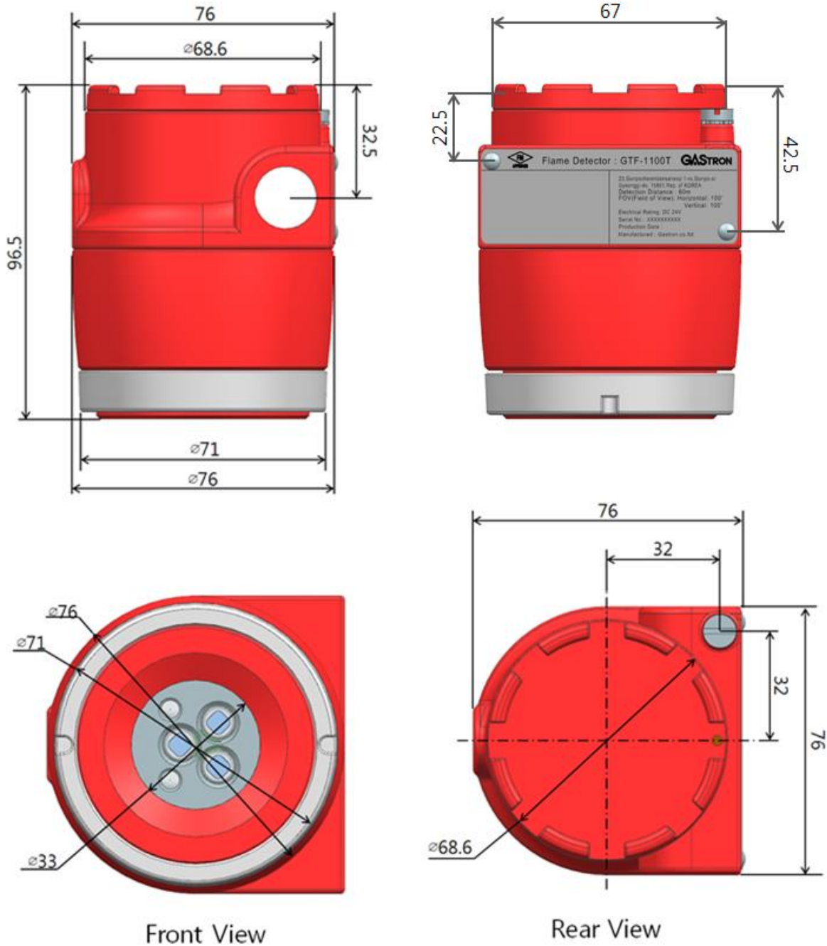
[Figure 11: GTF-1100T Dimensions]
