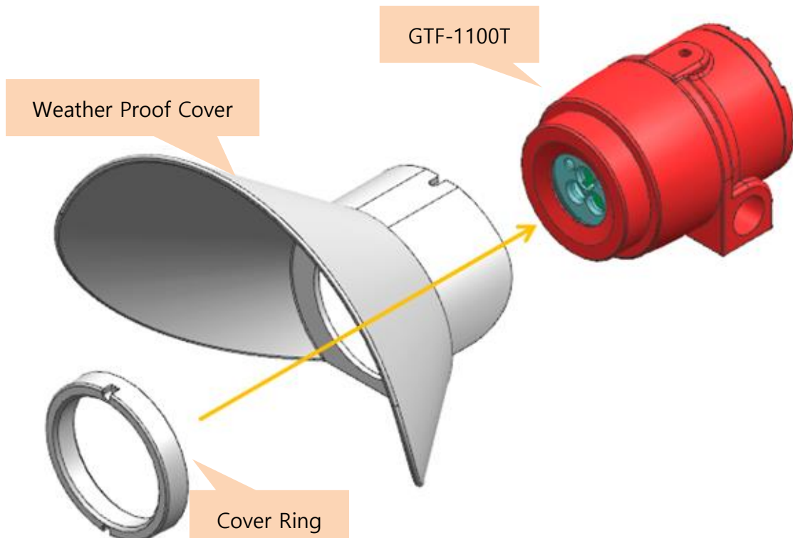
[Figure 17: Weather Proof Cover Assembly]
