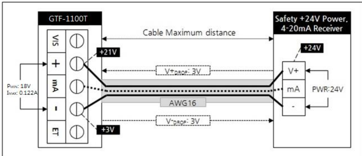
[Figure 5: Calculation of Length of GTF-1100T Cable Installation]
