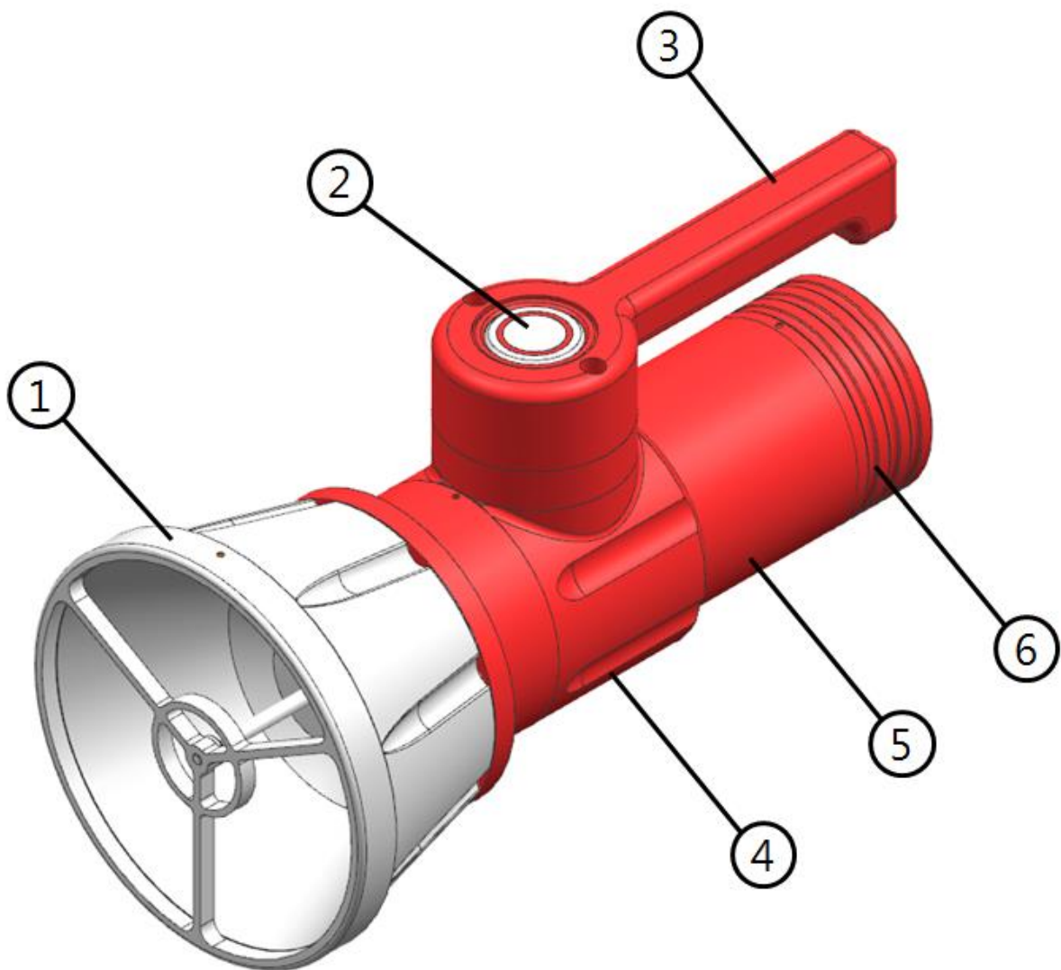
[Figure 15: Names of FS-320 Parts]
