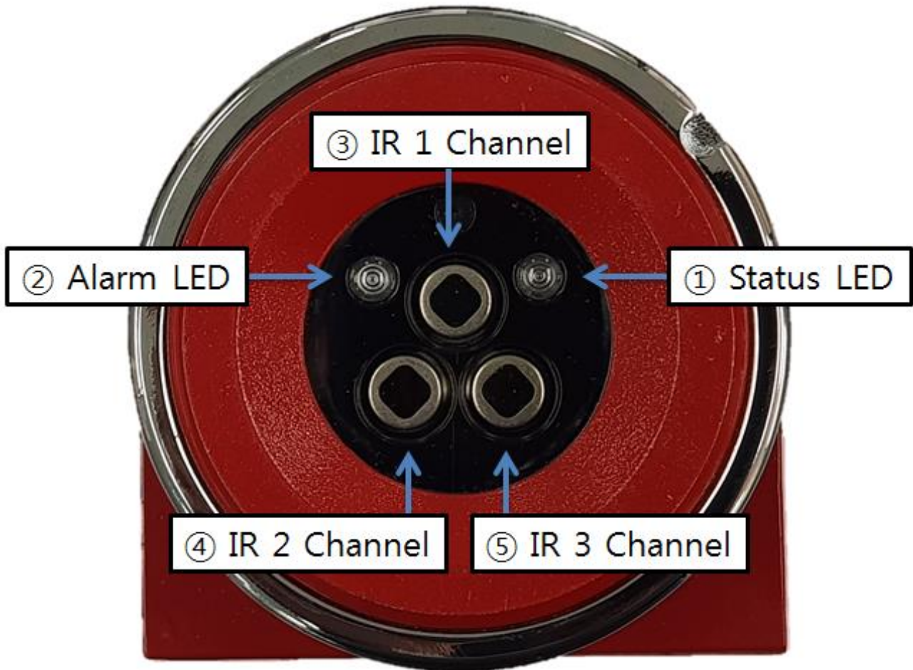
[Figure 9: Front Configuration]
