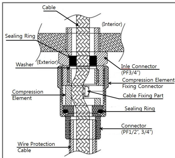
[Figure 21: Pressure Packing Type]
